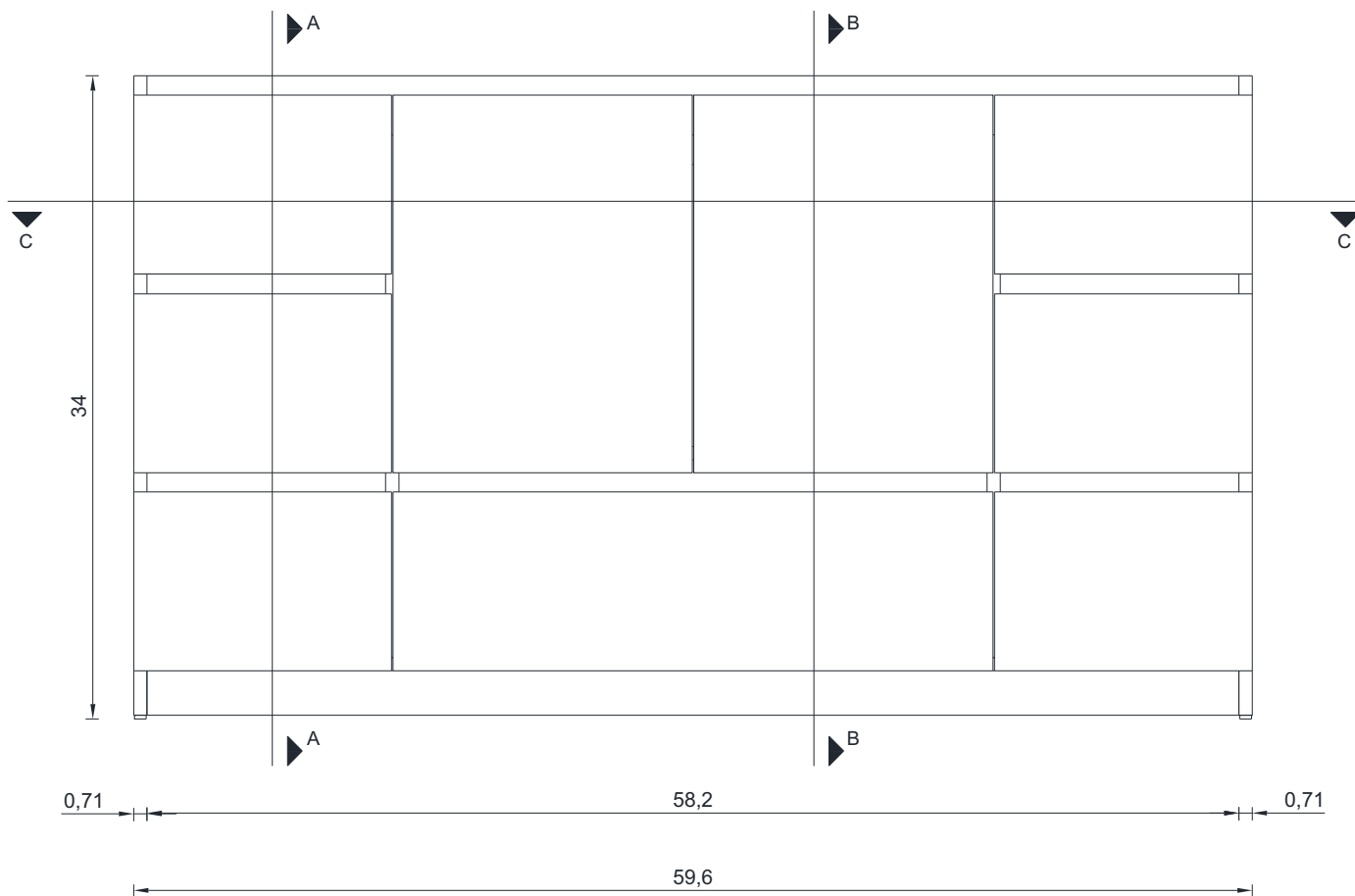
FRONT VIEW
