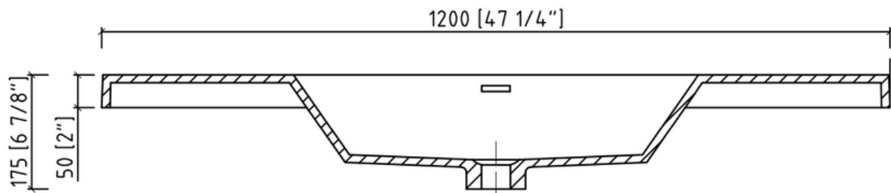
SECTION B-B
