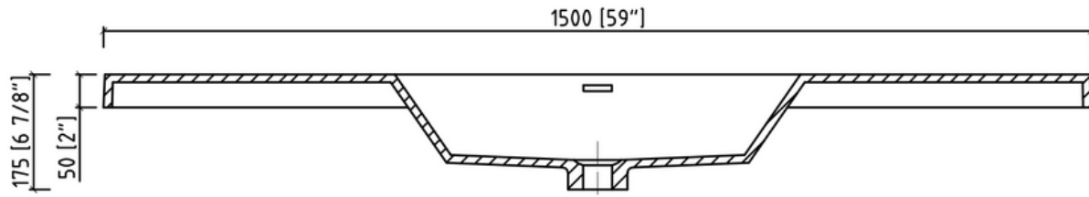
SECTION B-B
